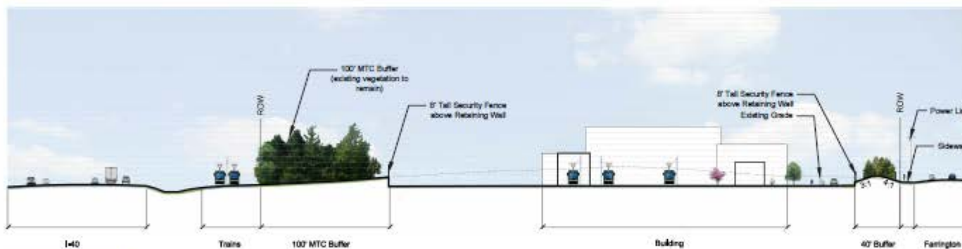
SITE SECTION B - VIEW TO THE SOUTH
